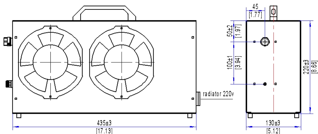
Outline B: With Fan
