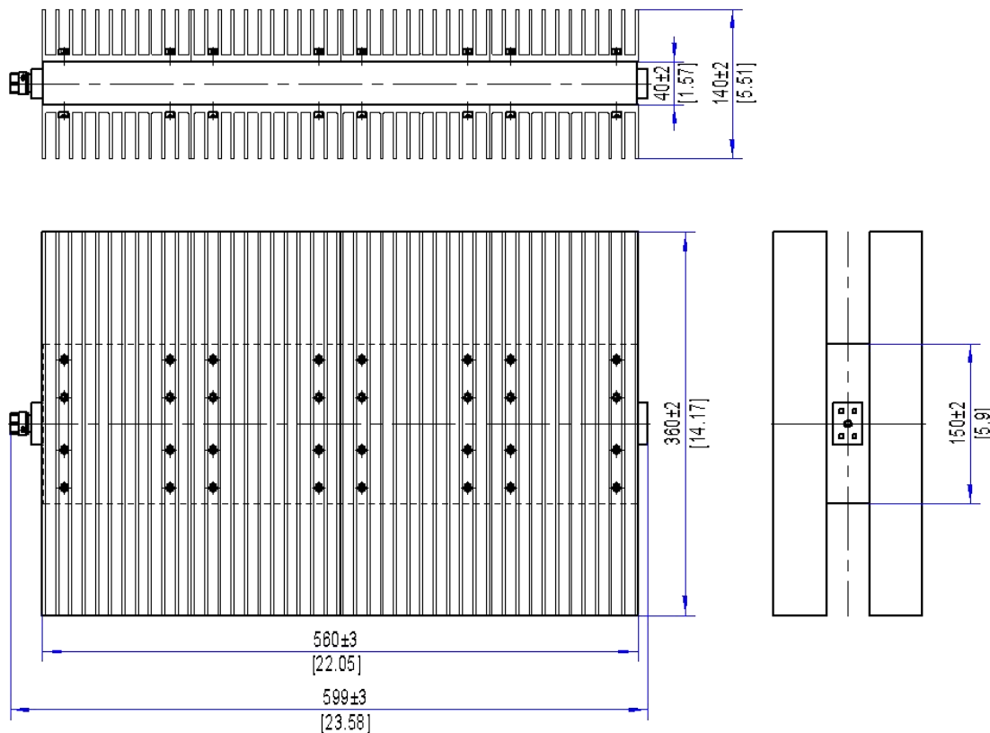
Outline A
