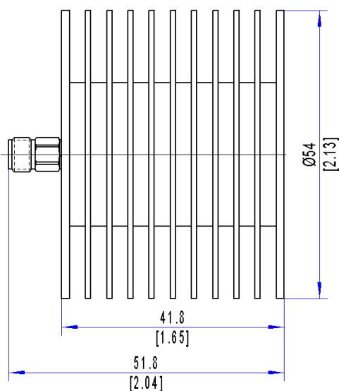
Outline A
