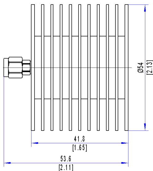
Outline B
