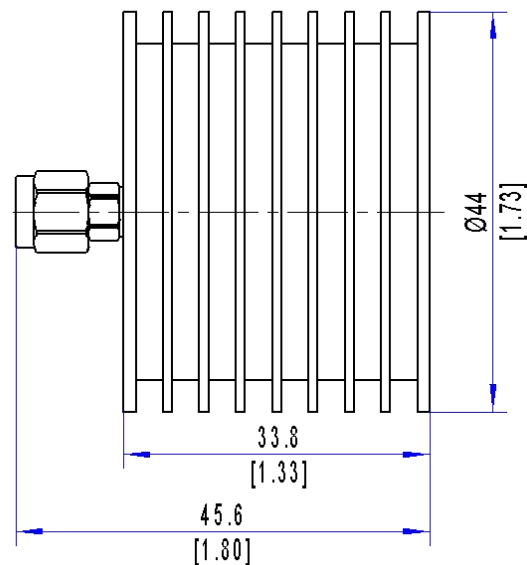
Outline B
